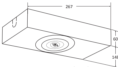
Dimensions (mm) SMS
