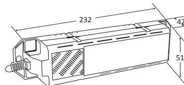
Dimensions (mm) Ballast
