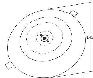
Dimensions (mm) With Adaptor Plate
